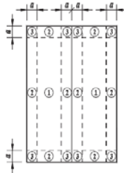
Wind Zones for Gable Roofs with 27° < \theta ≤ 45°:
